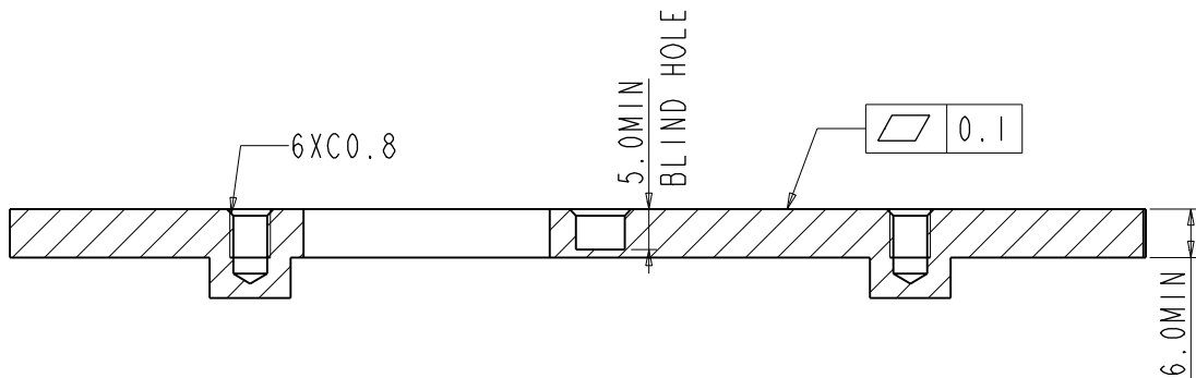
SECTION C-C
