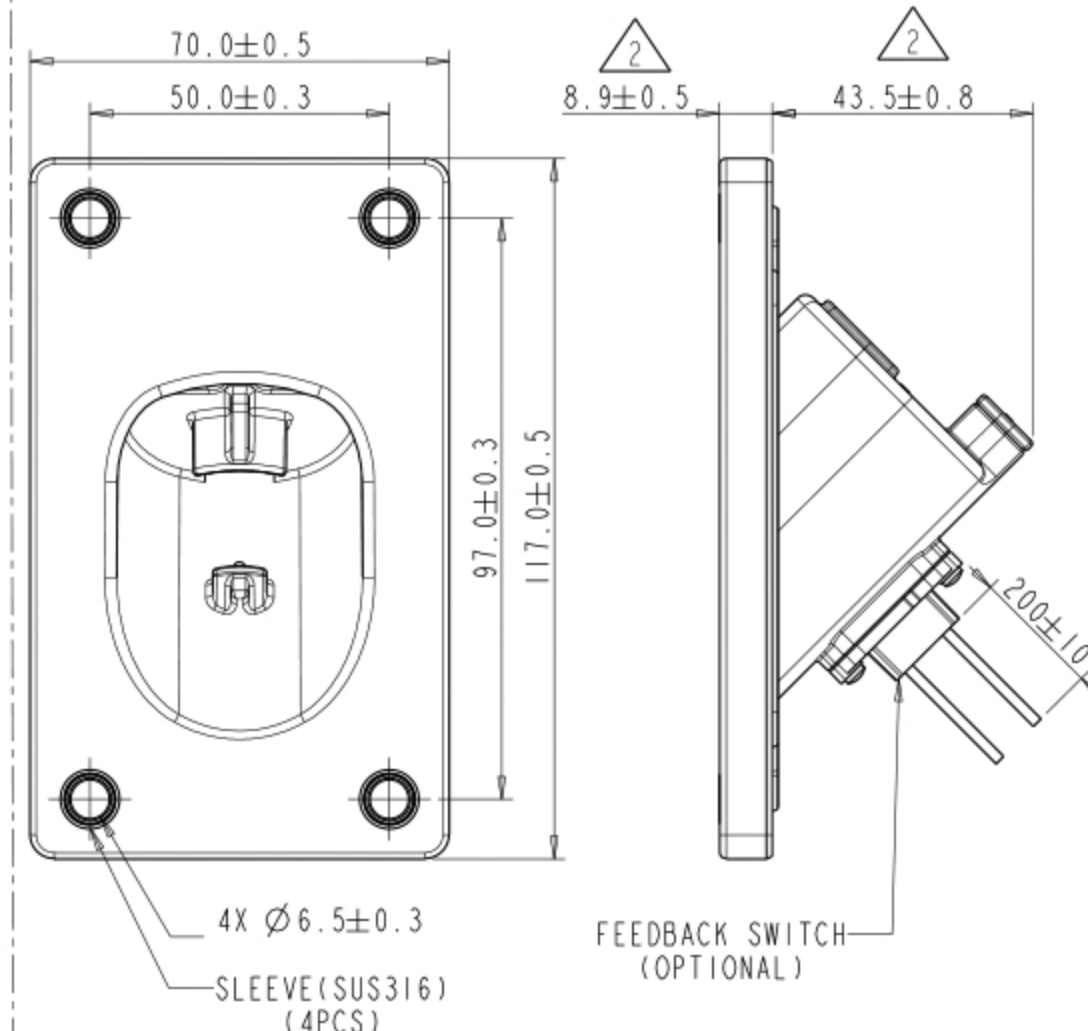
SLEEVE TYPE
