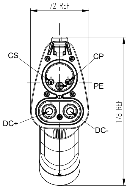
Front view of plug
