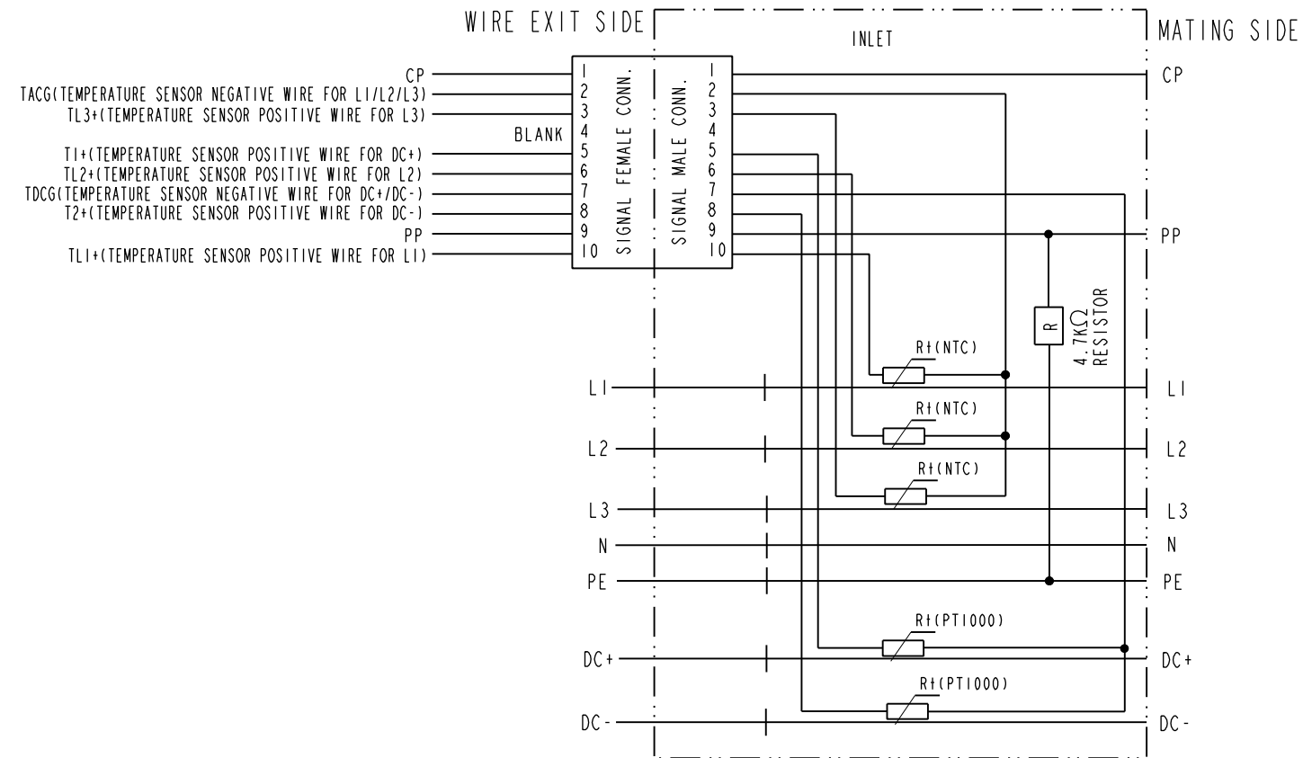
3-PHASE AC CHARGING AND DC CHARGING
