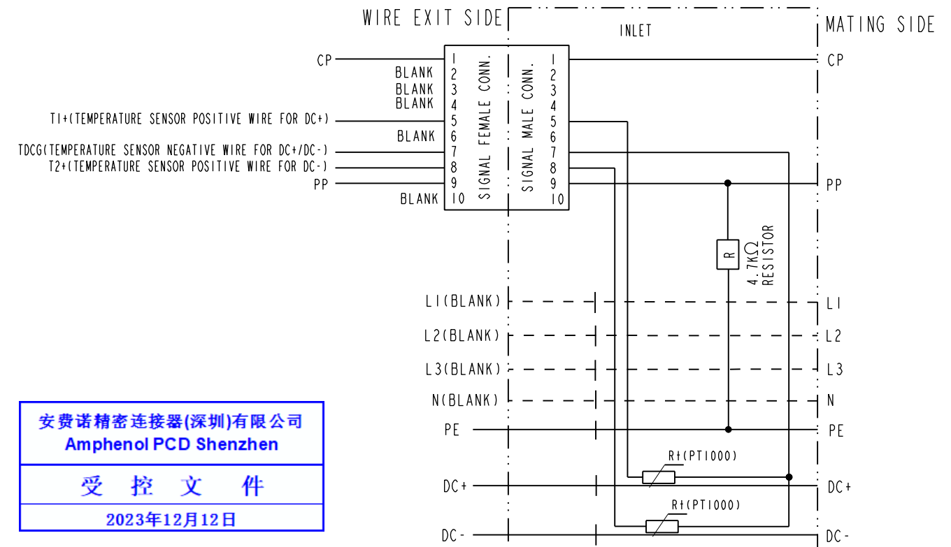
ONLY DC CHARGING
