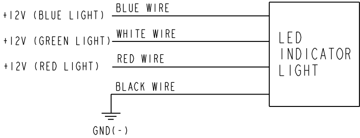
FIGURE 3 WIRE DIAGRAM FOR LED INDICATOR LIGHT
