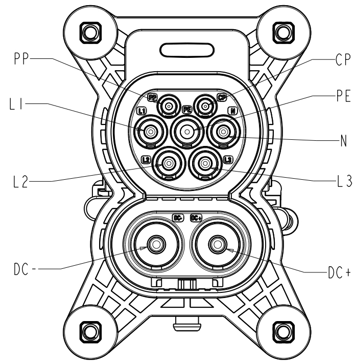
FIGURE 2 CABLE CONNECTING
