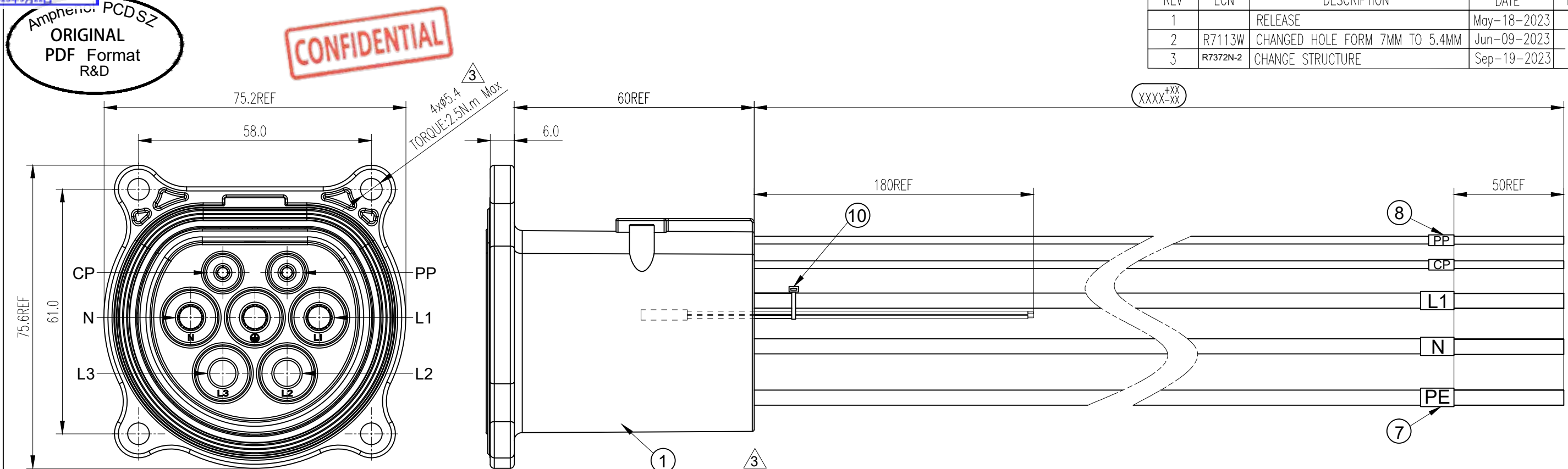
IEC SOCKET
