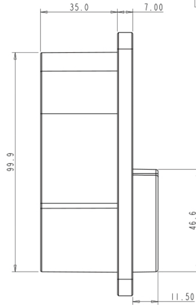
C220027208 WITHOUT DRAINAGE OUTLET
