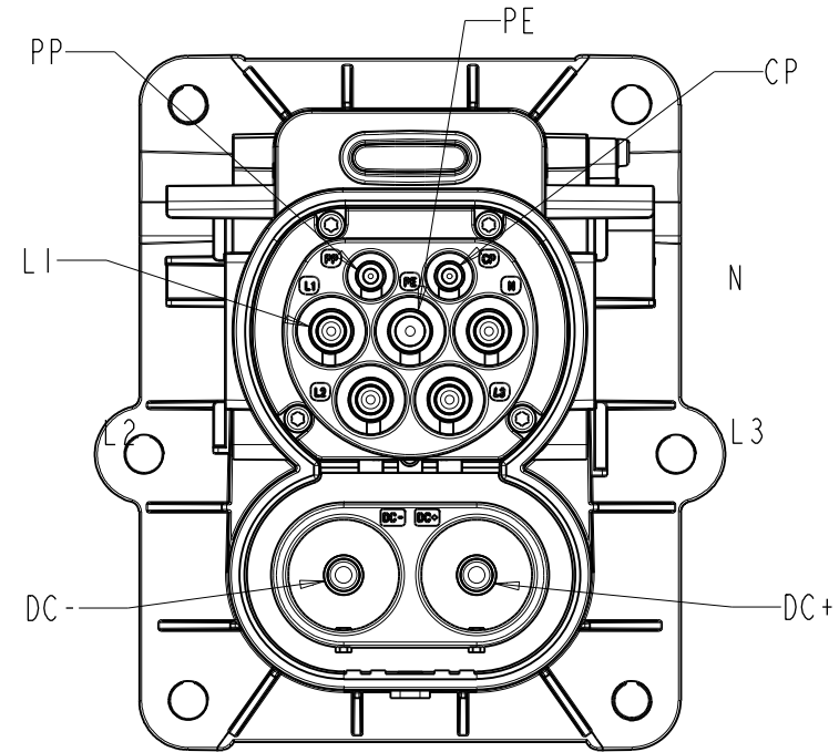
FIGURE 2 WIRING DIAGRAM FOR INLET
